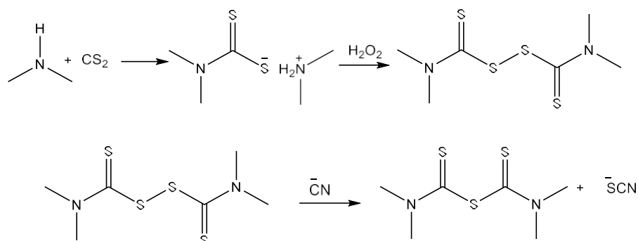
Fig. 5: Synthesis of TETS by heterolysis of disulfide bond with separation of thiocyanate ion
