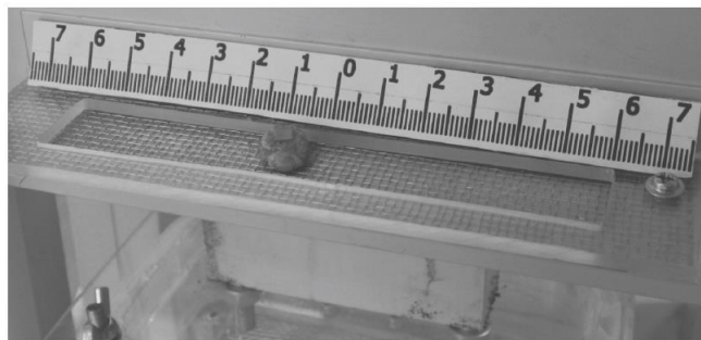
Fig. 5. Realized device with a wide range of possibilities that simulates the operation of a vibrating platform (5a), a mechanical model of the distribution of forces on a vibrating platform (5b) and a photographic representation of sand granules on a sieve (5c)
