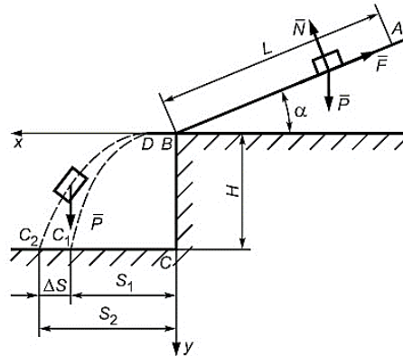
Fig. 4. Device for determining the dynamic coefficient of friction [3]
