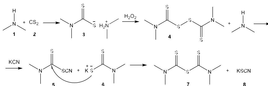
Fig. 7: Reaction mechanism of TETS synthesis
